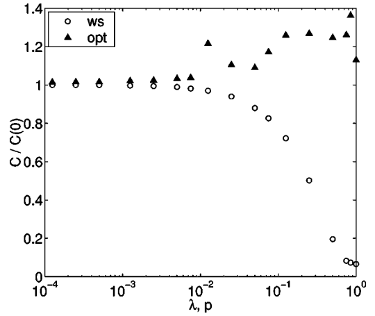
FIG. 6. Comparison between the WS model and the optimization model for a n=100, k=4 network, with respect to the variation in their normalized clustering coefficient C/C(0) . Both variations are averaged over 40 realizations.
